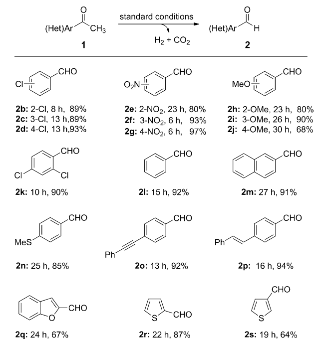
Scheme 1. Carbon–carbon bond cleavage of (hetero)aryl methyl ketones.
